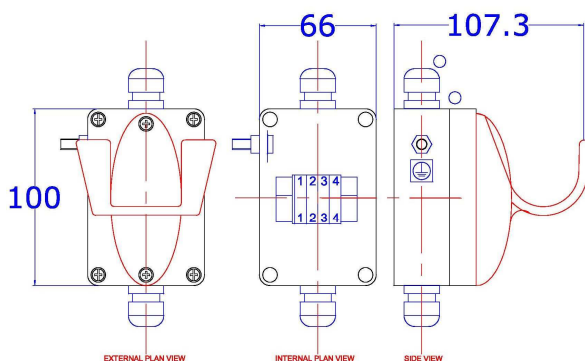
iSCAN100 Extender Junction Box
